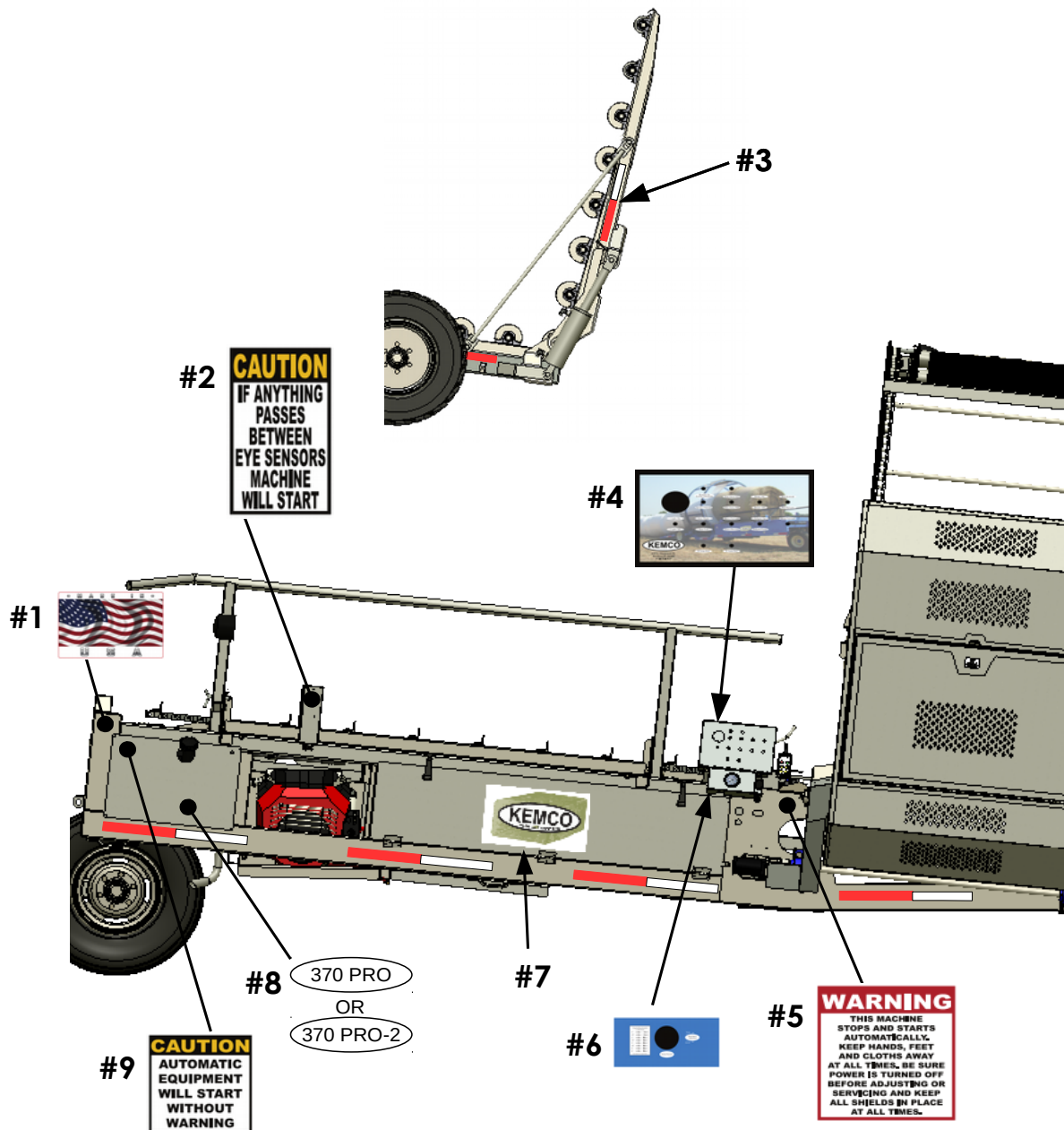
KEMCO MODEL 370 DECALS, MACHINE SIDES
