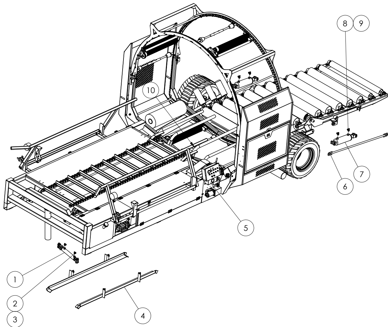
KBW MODEL 370 MISC. REMOVABLE PARTS
