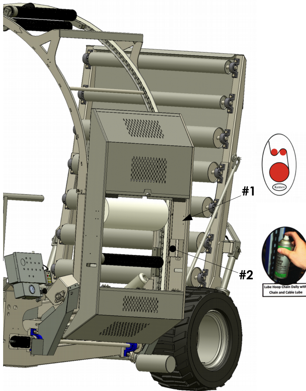
KEMCO MODEL 370 DECALS, WRAP MAINTENANCE
