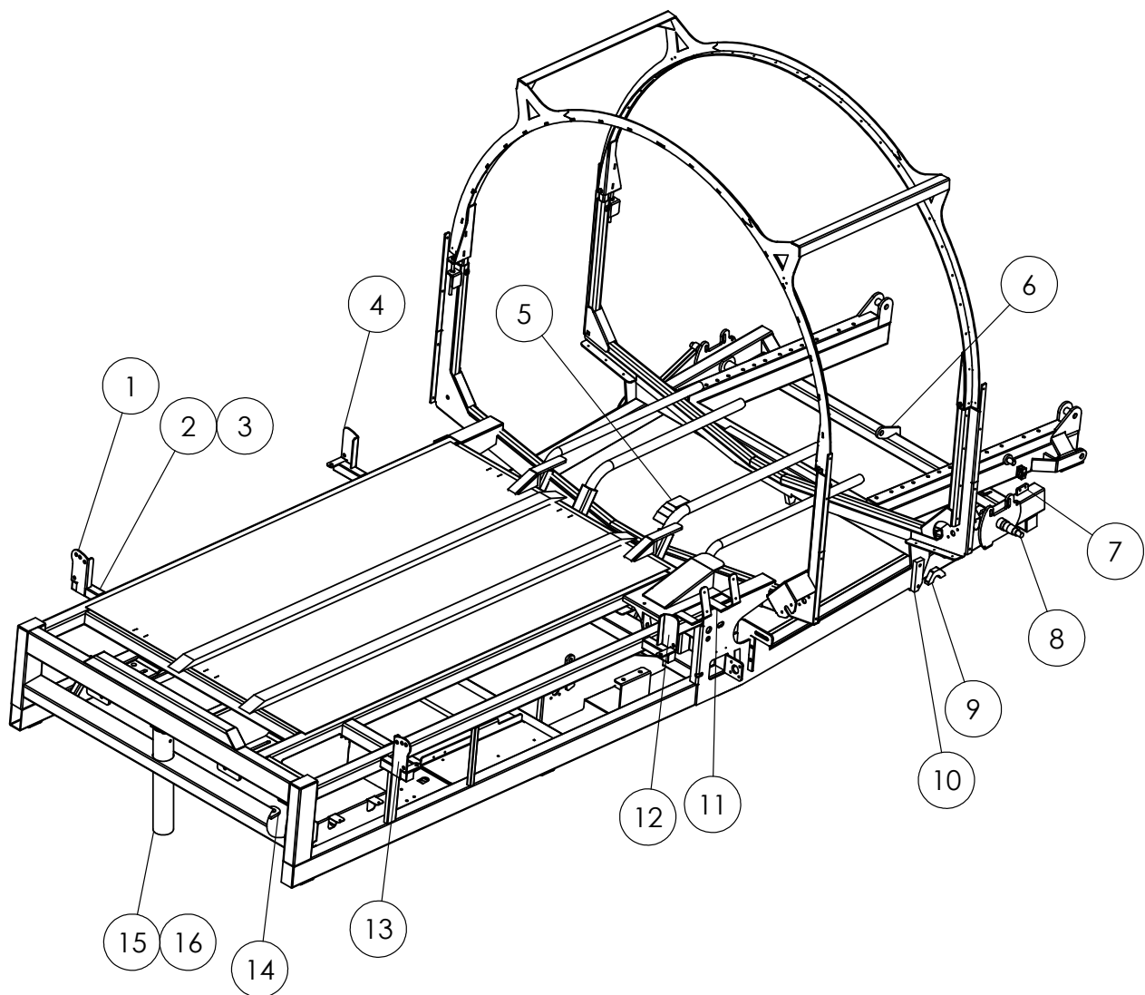
KBW MODEL 370 CHASSIS WELD PARTS
